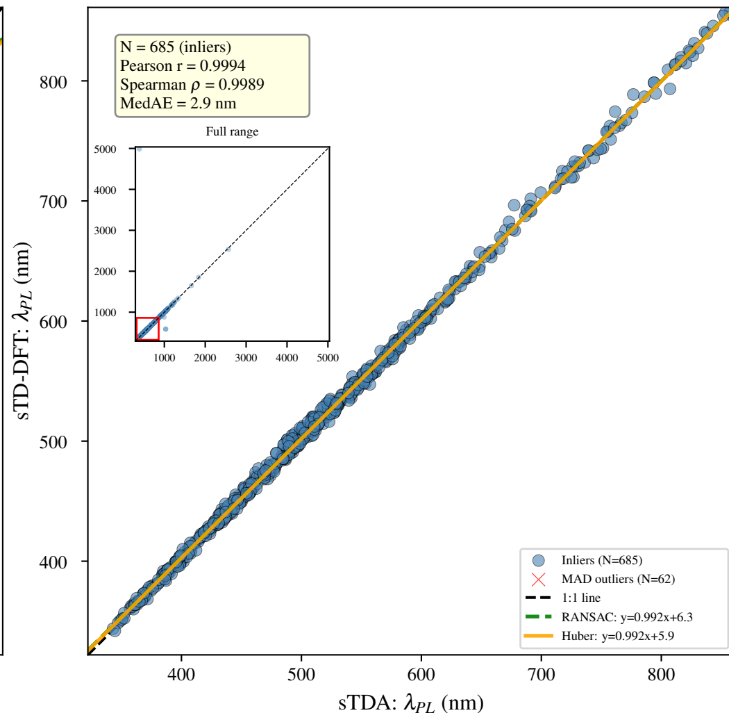
\lambda_{PL} (nm) - Gas Phase
