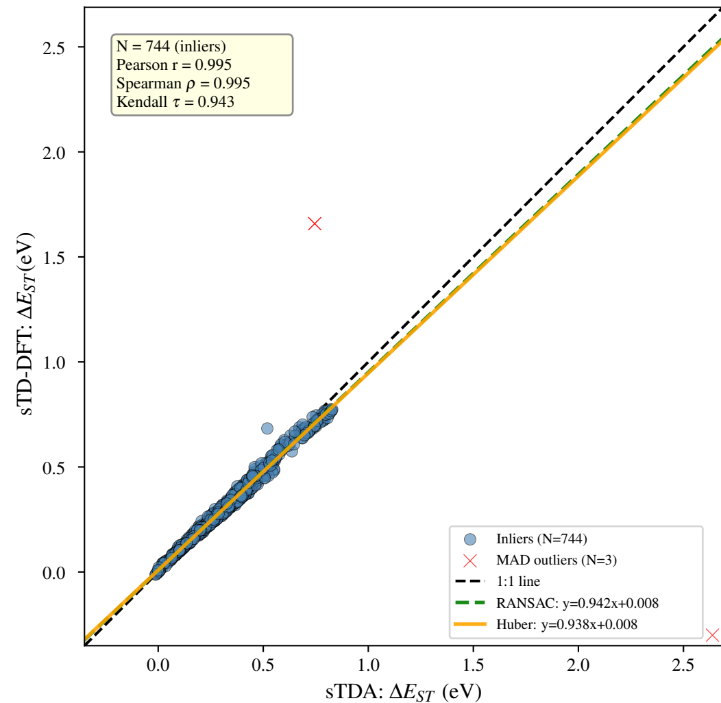
\Delta E_{ST} (eV) - Gas Phase
